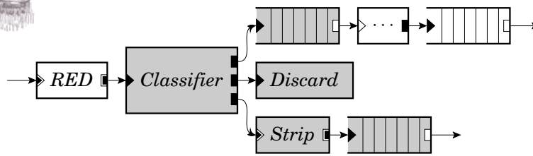
Fig. 5. Flow-based router context. A packet starting at RED and stopping at the first Queue it encountered might pass through any of the grey elements.
