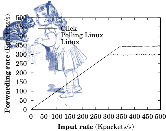
Fig. 17. Forwarding rate as a function of input rate for Click and Linux IP routers (64-byte packets).
