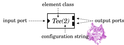
Fig. 1. A sample element. Triangular ports are inputs and rectangular ports are outputs.
